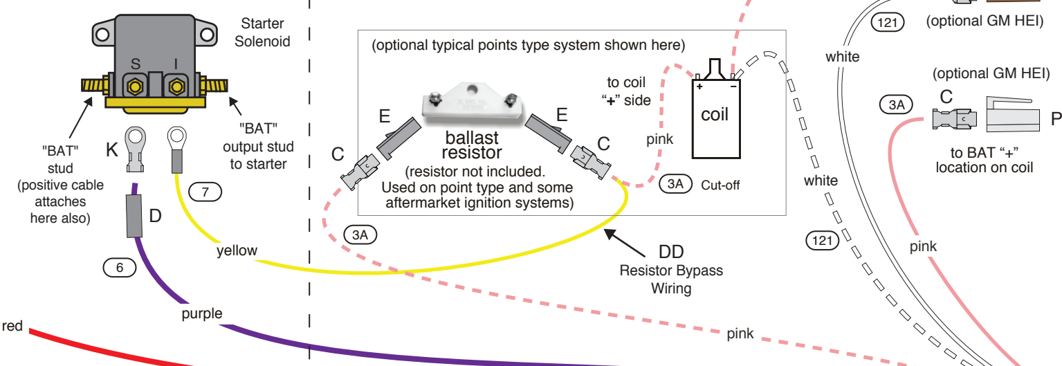
Figure "B" Ignition, engine sensors, electric choke, washer pump, tach, electric speedometer and brake switch
